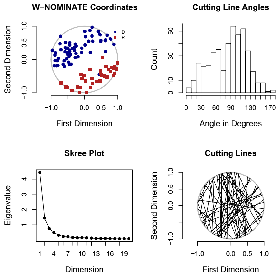
Figure 1: Summary Plot of 90th Senate W-NOMINATE Scores
